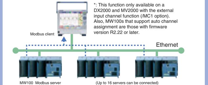
MW100 Modbus server (Up to 16 servers can be connected)
