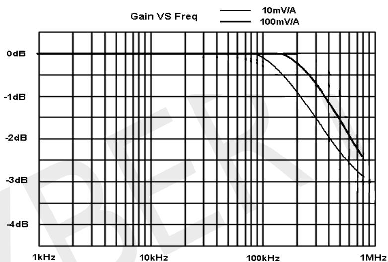
Figure 1 CPL8100A Typical Gain VS Frequency curve
